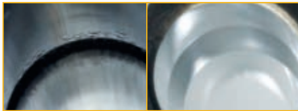
The forcing cone of the competition's barrel is pitted and damaged beyond repair after 500 rounds of steel shot.
