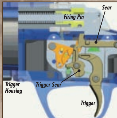
Full sear engagement (Ready to fire)
