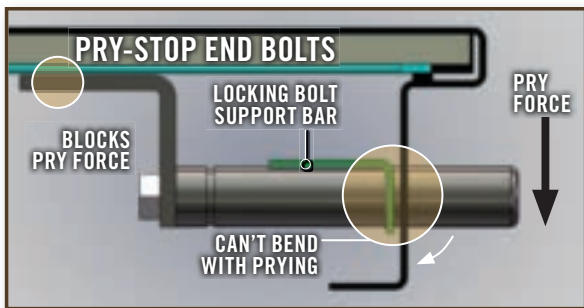
Pry-Stop End Bolt Mechanism secures door corners in a pry attack.
