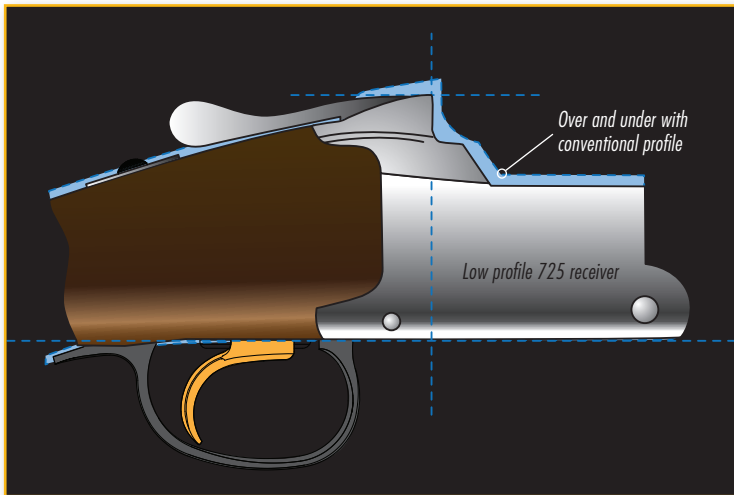
Improved recoil control and less muzzle jump are two of the big benefits of a low-profile receiver. There is also the "one with the gun" feeling that makes the shotgun act like an extension of your body.
